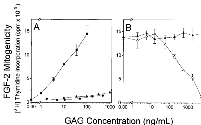
FIG. 3. Mitogenic activity of FGF-2 in the absence (A) and presence (B) of added heparin. Heparin (■), N -sulfoacharan sulfate (▲), syndecan-1 (●), and acharan sulfate (△) were used at increasing concentrations and the incorporation of [^3\text{H}] -thymidine into DNA by F32 cells was measured. The heparin (alone) and FGF-2 (alone) controls gave \sim 750 cpm.
